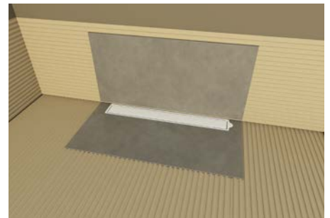
9. Set tiles up to the edge of the protection cover
