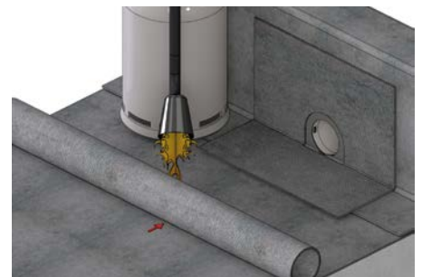
9. Set second horizontal bitumen layer
