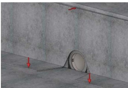
10. Set second vertical bitumen layer
