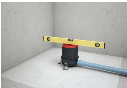
4. Adjust the decline of the pipe by using the angles and level the drain body.
