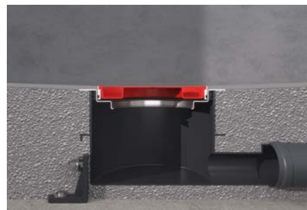
15. Flush finish of the coating with the round stainless steel frame.
